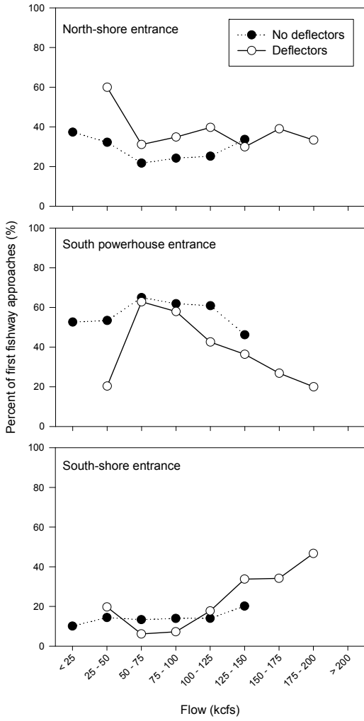
Figure 14. Percentages of total fishway approaches as distributed among fishway entrances, by flow and presence or absence of spill defectors.
