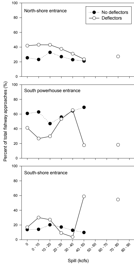
Figure 13. Percentages of total fishway approaches as distributed among fishway entrances, by spill and presence or absence of spill deflectors.
