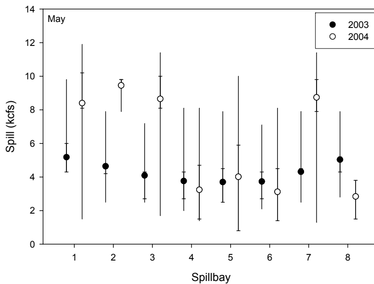
Figure 7. Mean, quartile, and 5 th and 95 th percentiles of spill recorded passing through each spillbay in May of 2003 and 2004. Spill occurred during 96-99% of possible 5-minute periods for each spillbay in 2003 and during 6-49% of periods in 2004.
