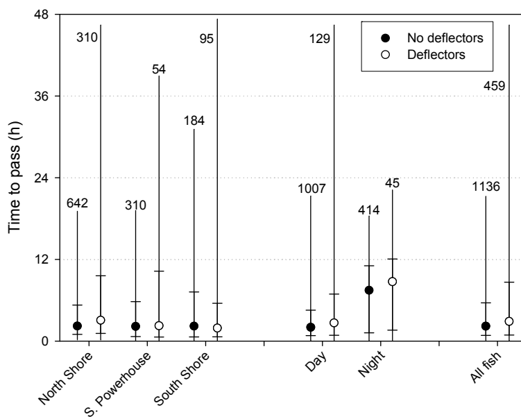
Figure 31. Median, quartile, and 5 th and 95 th percentiles of Chinook salmon passage times from first recorded fishway approach to first fishway entry. Categories are location of first approach, day vs. night, and all fish during the pre- and post-spillway deflector periods.
