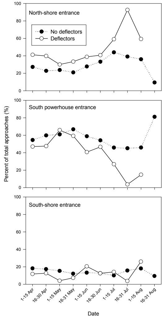
Figure 15. Percentages of total fishway approaches as distributed among fishway entrances, by date and presence or absence of spill defectors.
